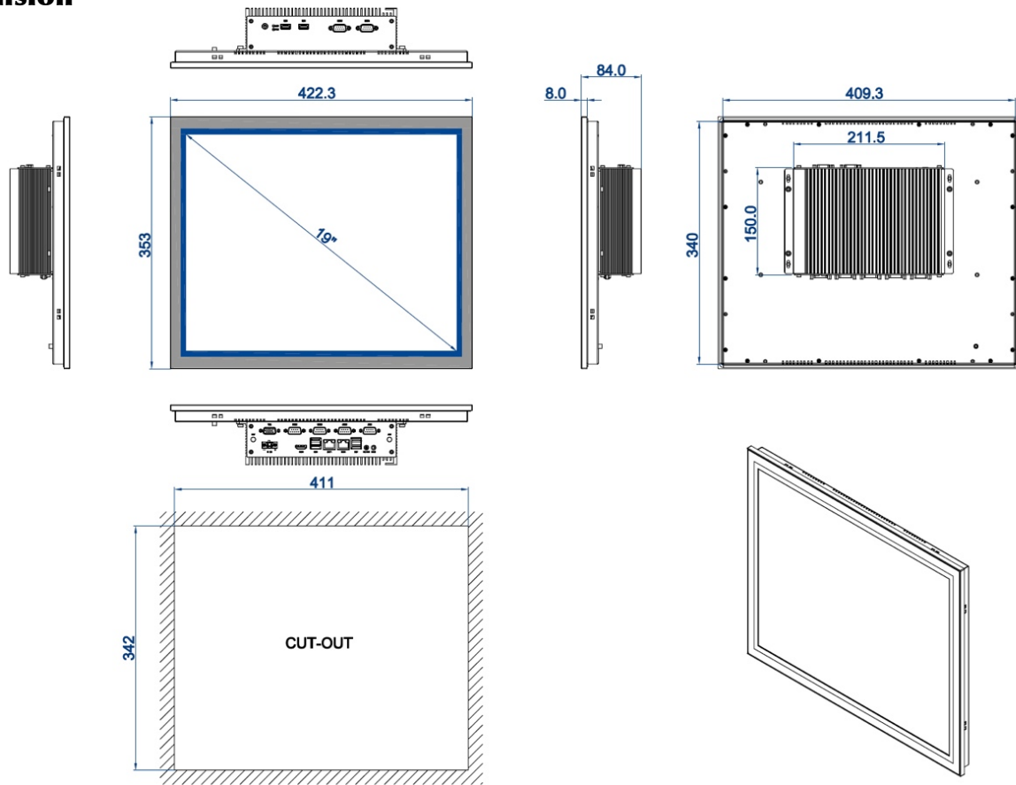
DIMENSIONAL DRAWING:TPC-PR190
