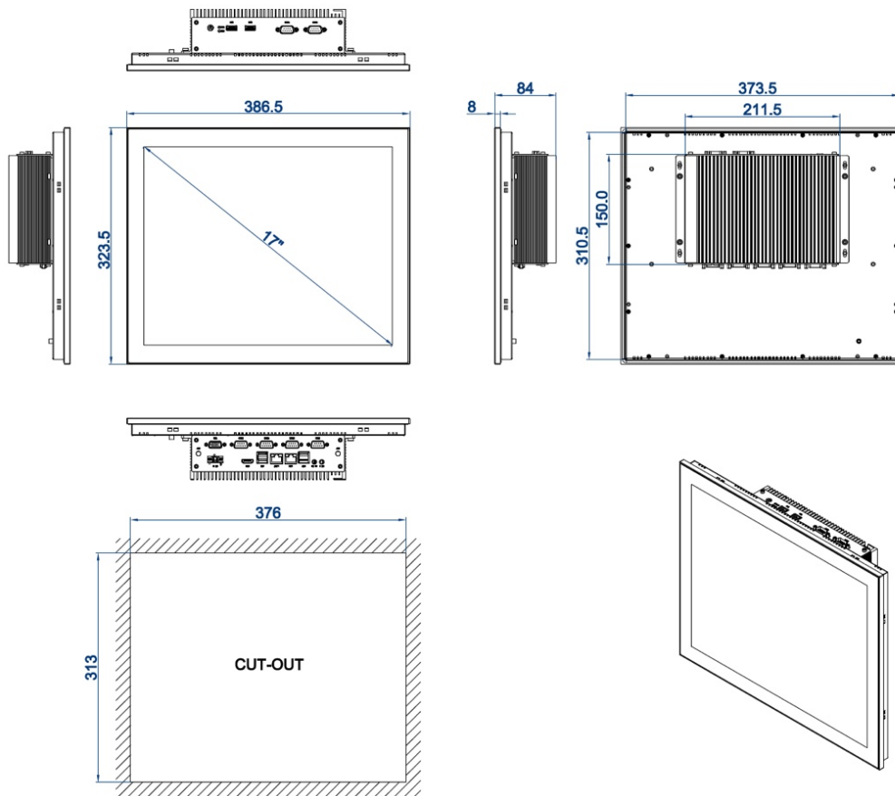
DIMENSIONAL DRAWING:TPC-PC170
