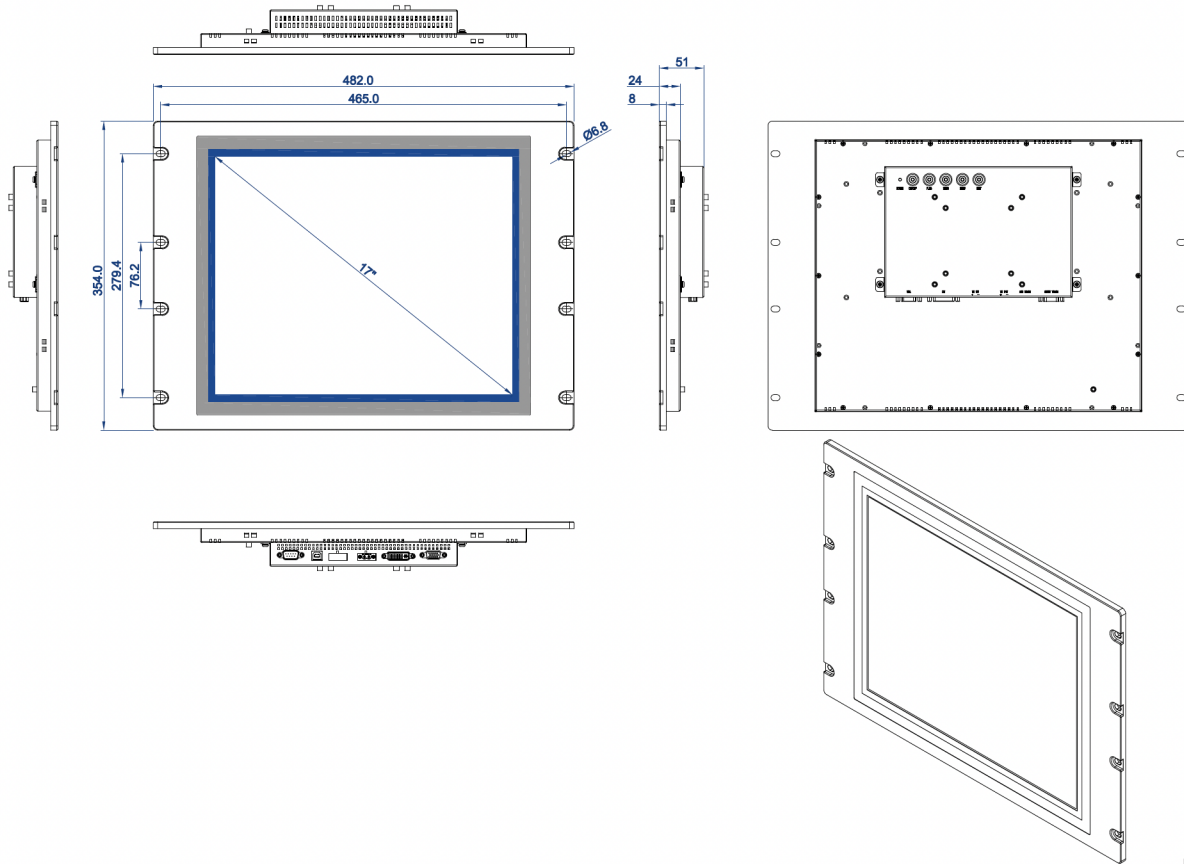
DIMENSIONAL DRAWING:TM-RR170
