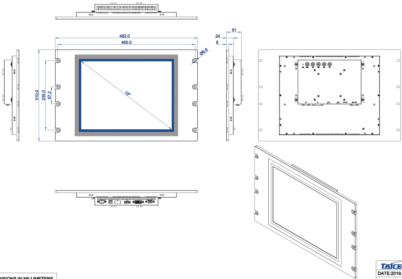
DIMENSIONAL DRAWING:TM-RR150
